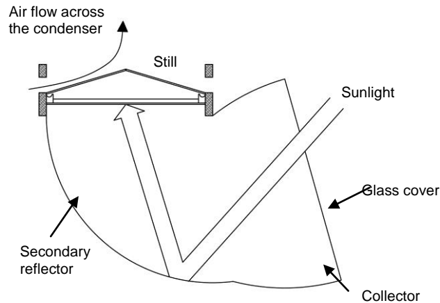
Figure 1: An inverted absorber solar still. Illustration: Neil Noble / Practical Action.
